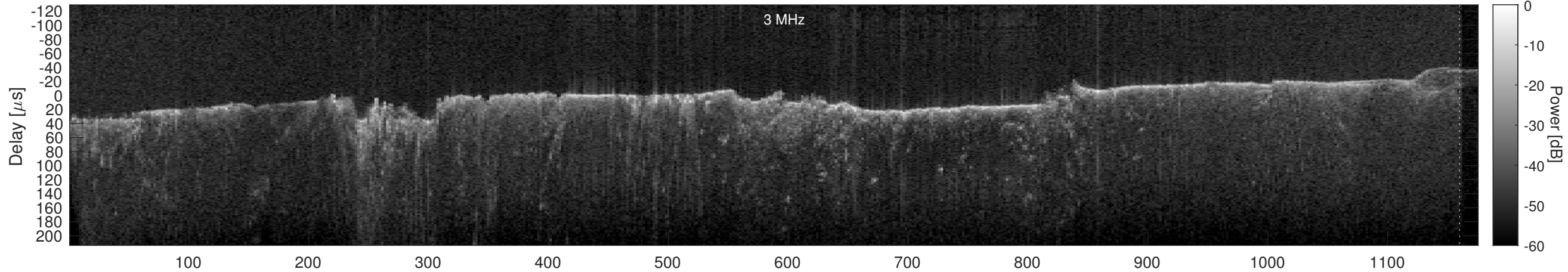
Orbit 2854, Cluttergram
