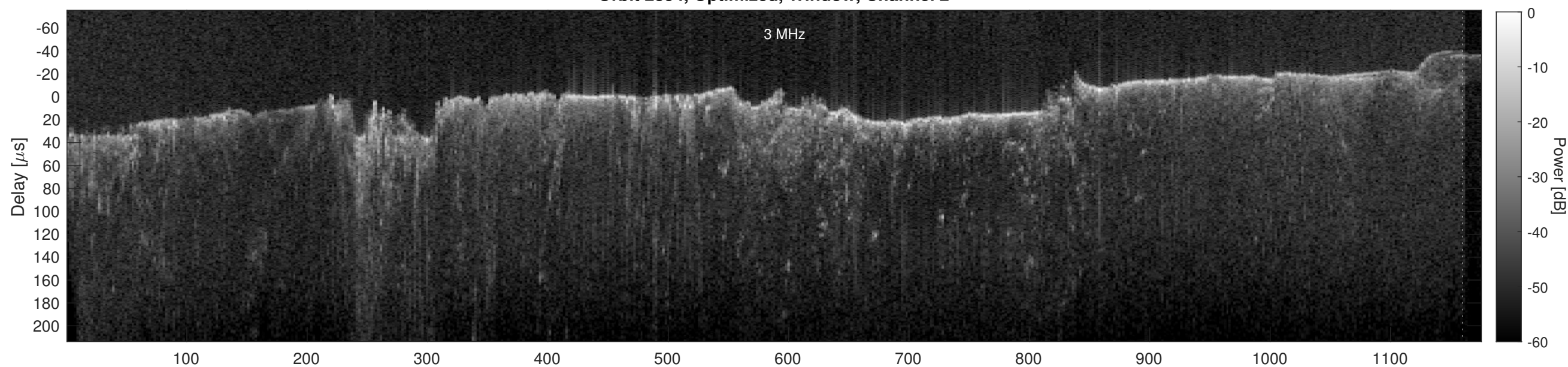
Orbit 2854, Cluttergram
