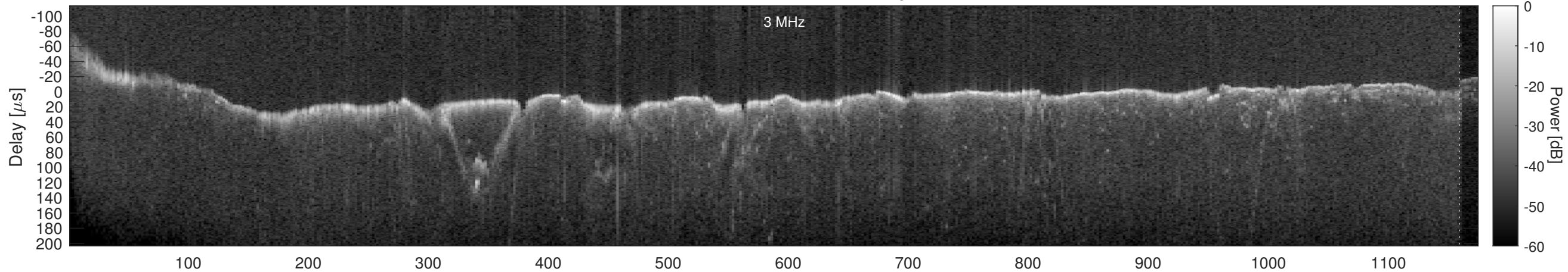
Orbit 2855, Window, Channel 2, Optimized
