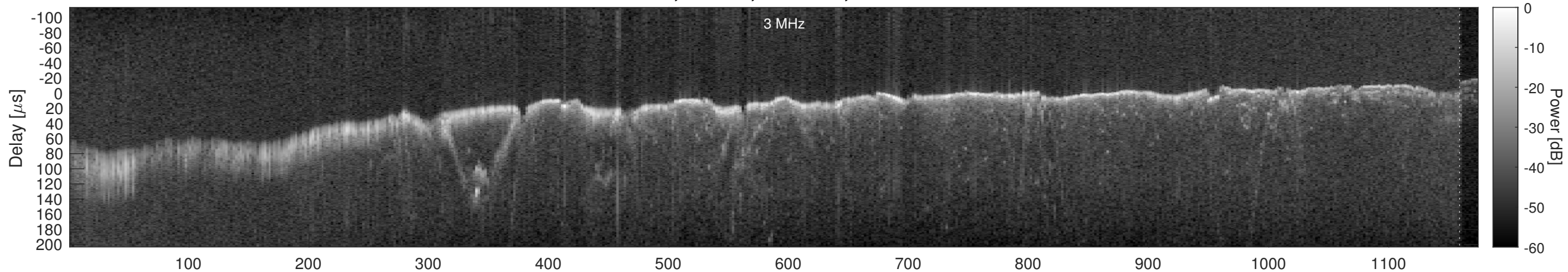
Orbit 2855, Window, Channel 2, Chapman
