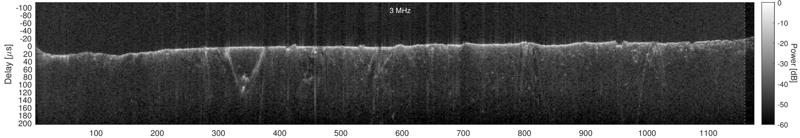
Orbit 2855, Cluttergram
