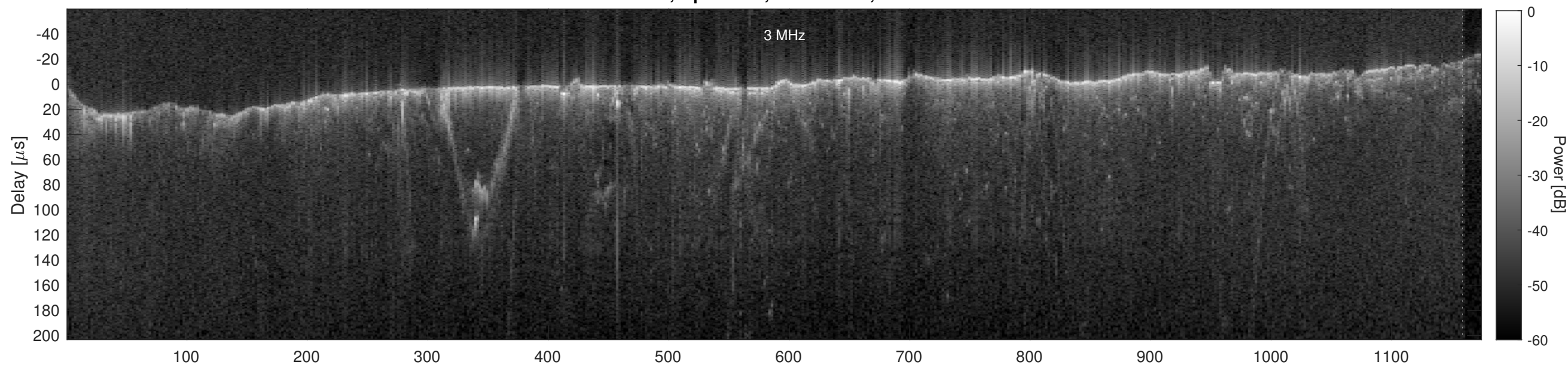
Orbit 2855, Cluttergram
