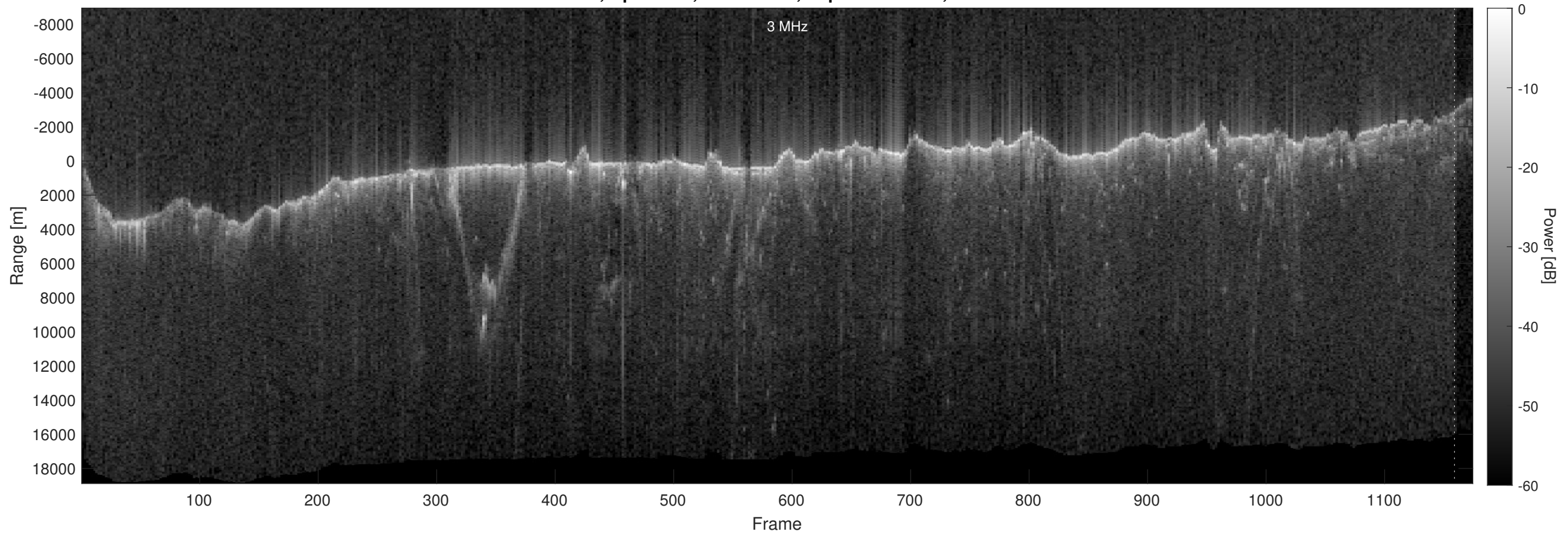
Orbit 2855, Optimized, No Window, Depth-Corrected, Channel 2
