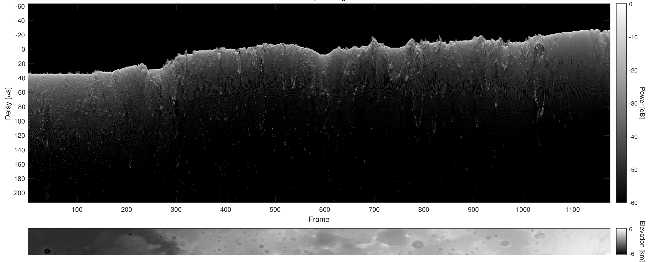
Orbit 2859, Cluttergram
