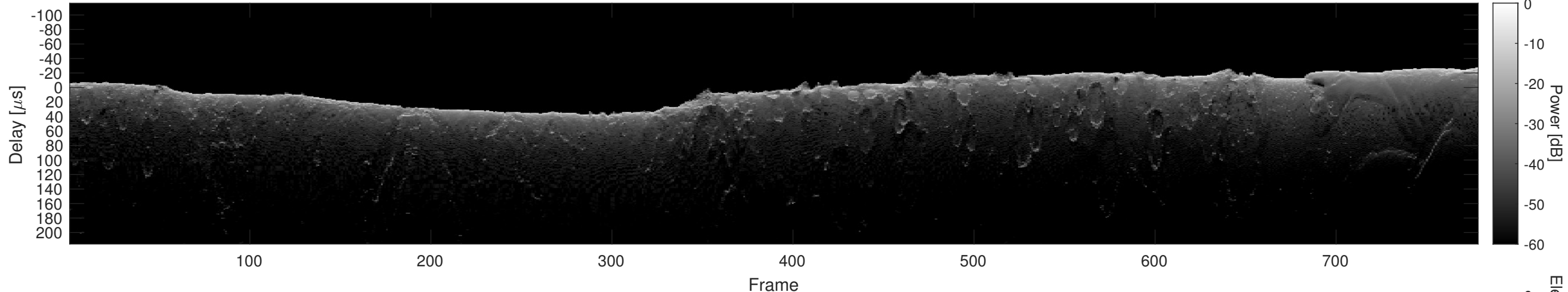
Orbit 2860, Cluttergram
