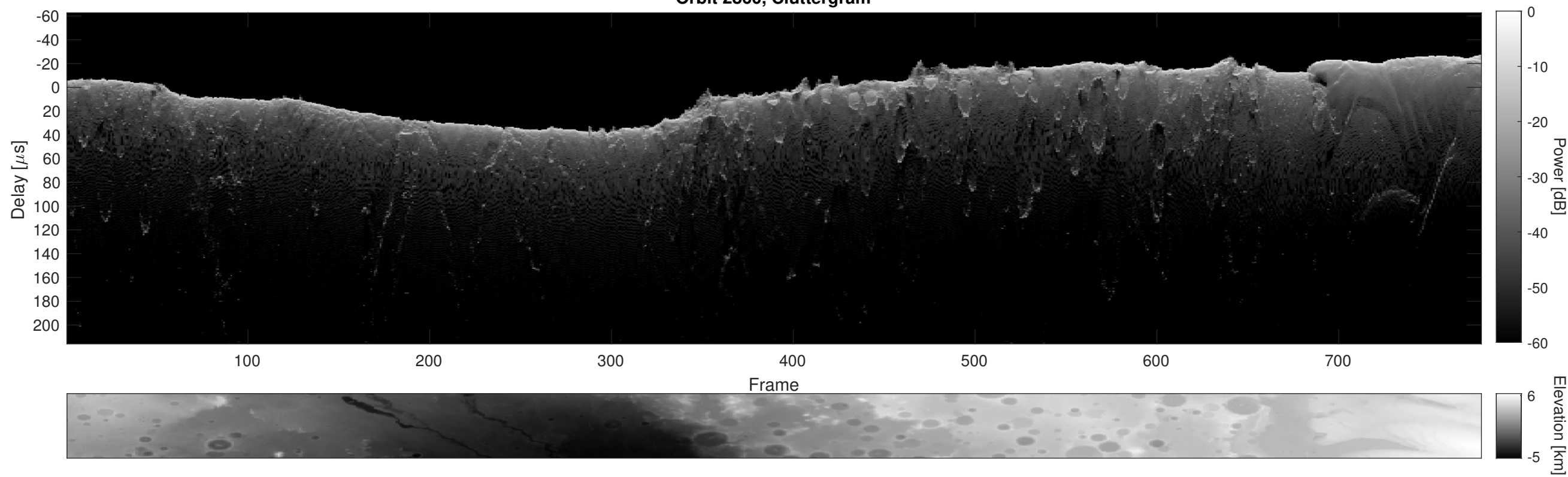
Orbit 2860, Cluttergram
