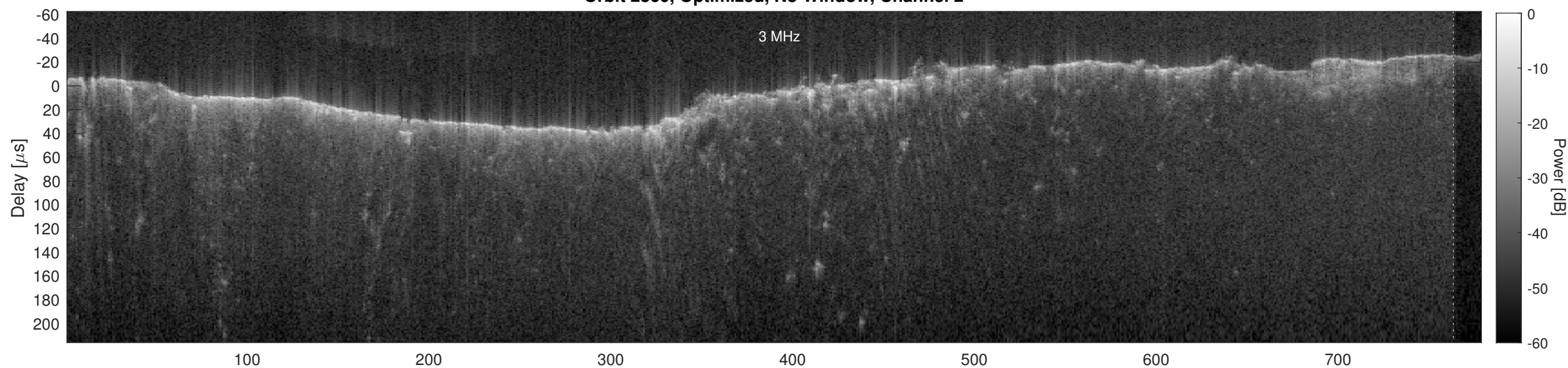
Orbit 2860, Cluttergram
