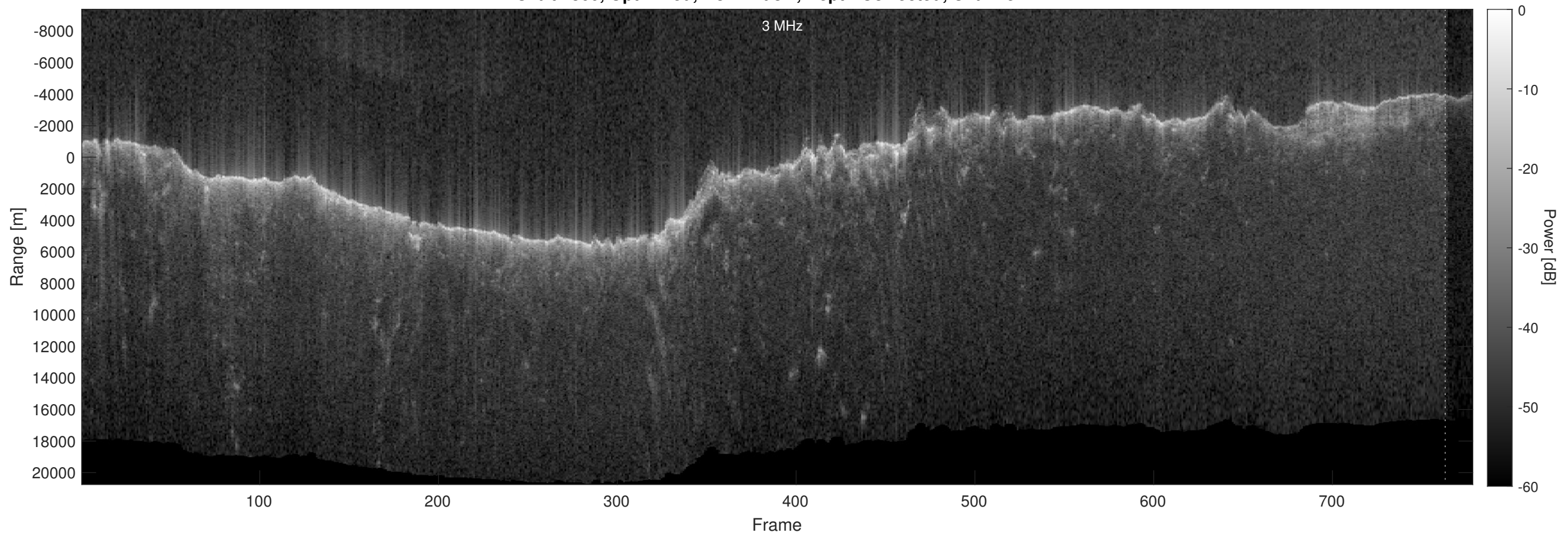
Orbit 2860, Optimized, No Window, Depth-Corrected, Channel 2
