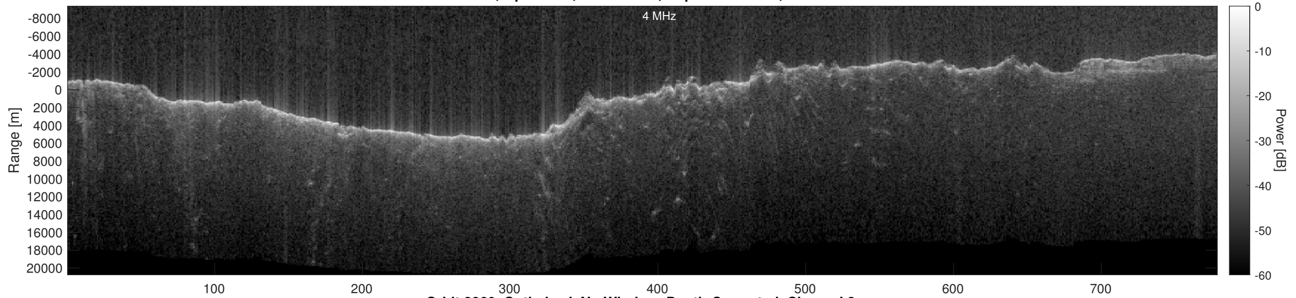
Orbit 2860, Optimized, No Window, Depth-Corrected, Channel 2
