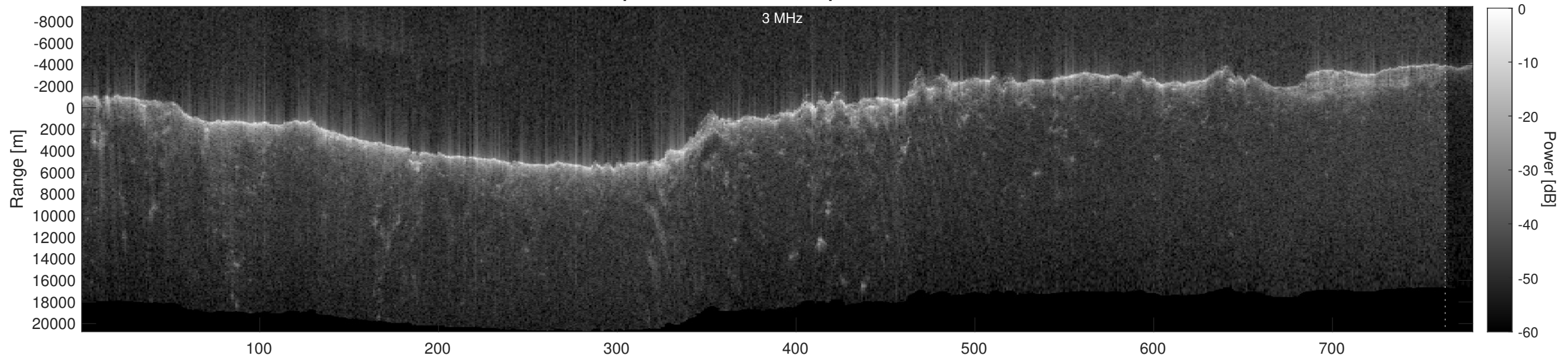
Orbit 2860, Depth-Corrected Cluttergram
