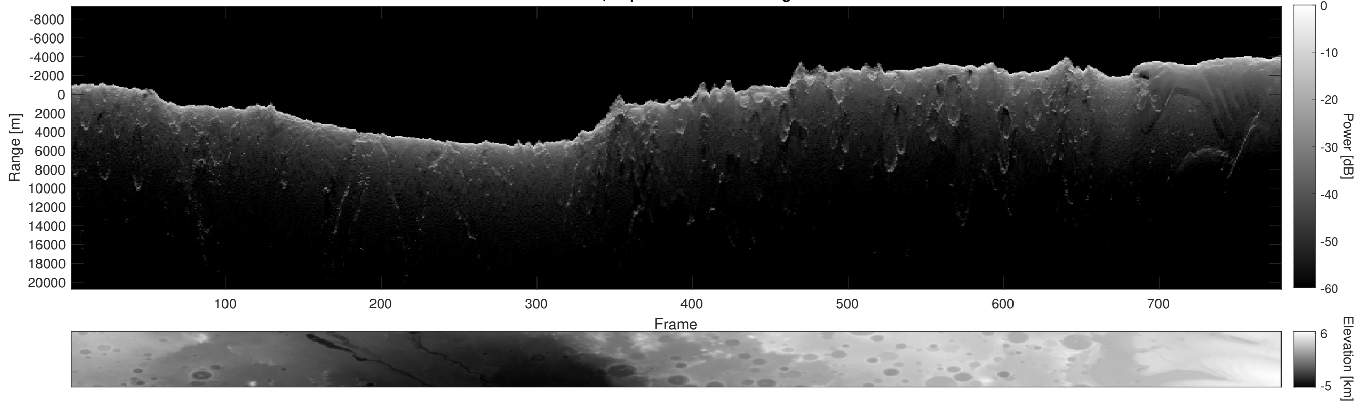
Orbit 2860, Depth-Corrected Cluttergram
