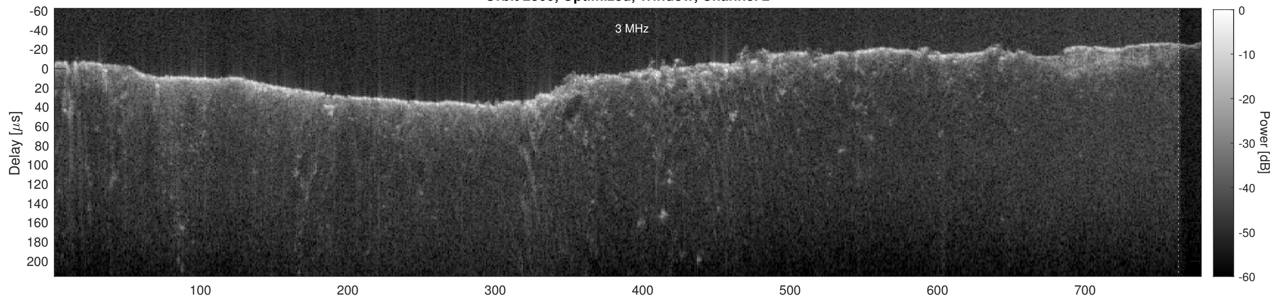
Orbit 2860, Cluttergram
