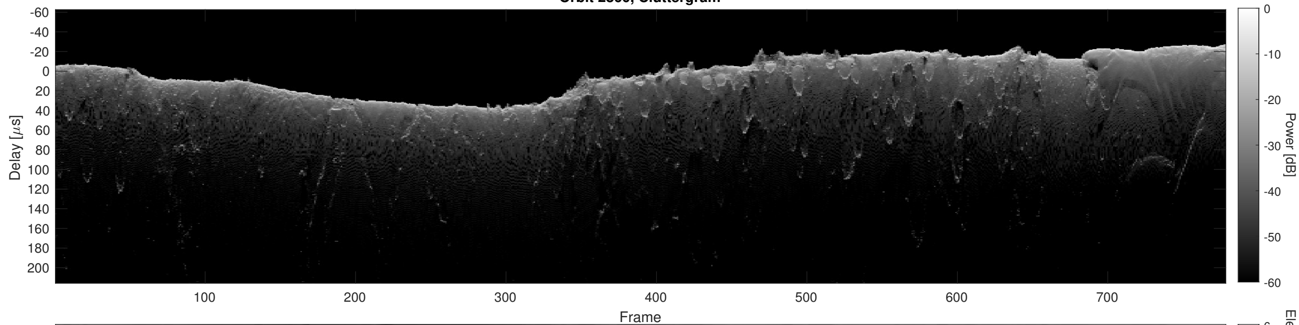
Orbit 2860, Cluttergram
