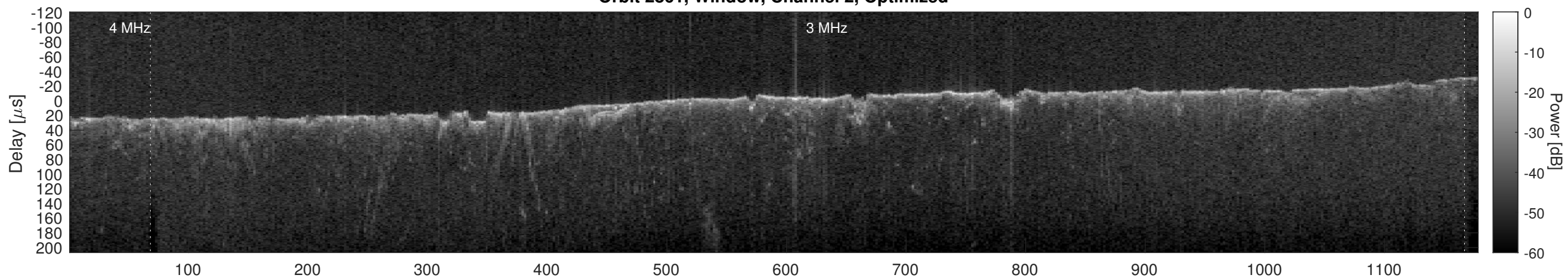
Orbit 2861, Cluttergram
