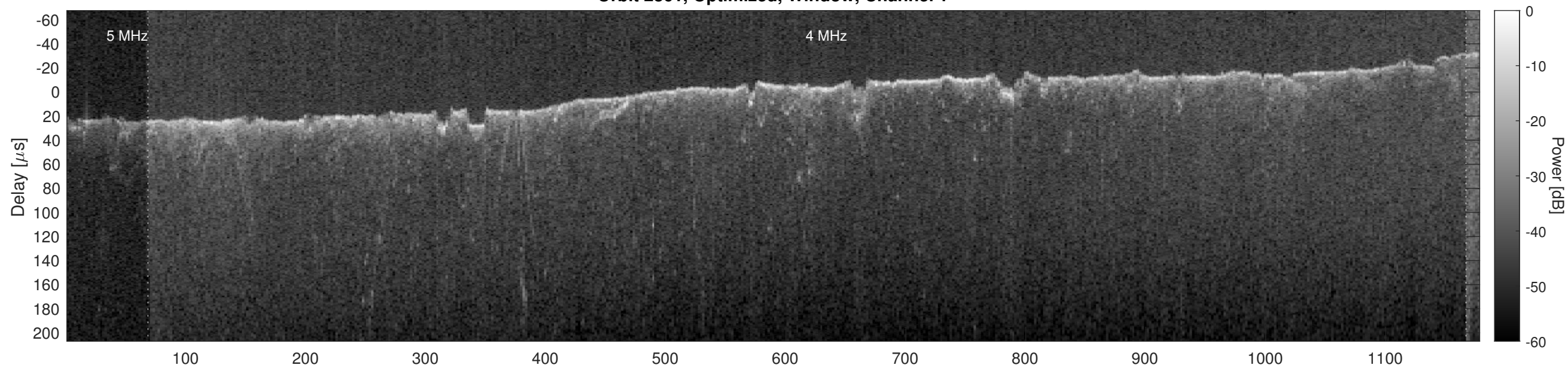
Orbit 2861, Optimized, Window, Channel 2
