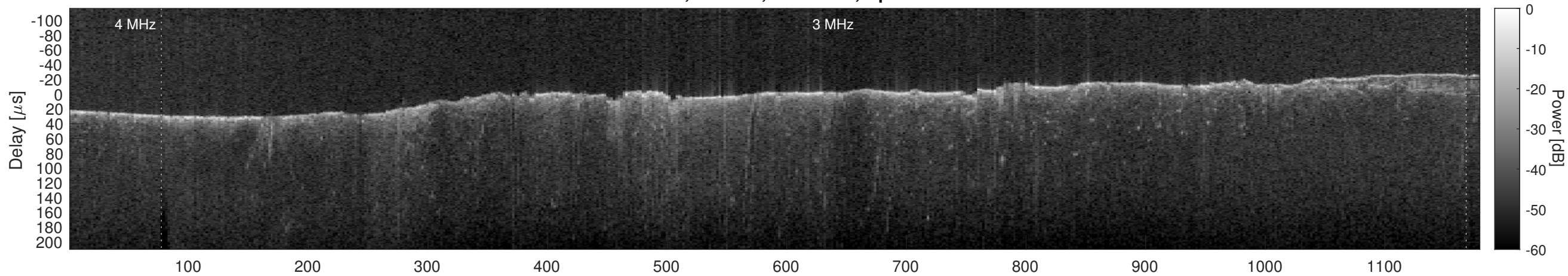
Orbit 2863, Cluttergram
