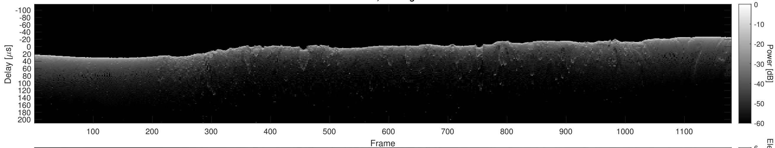
Orbit 2863, Cluttergram
