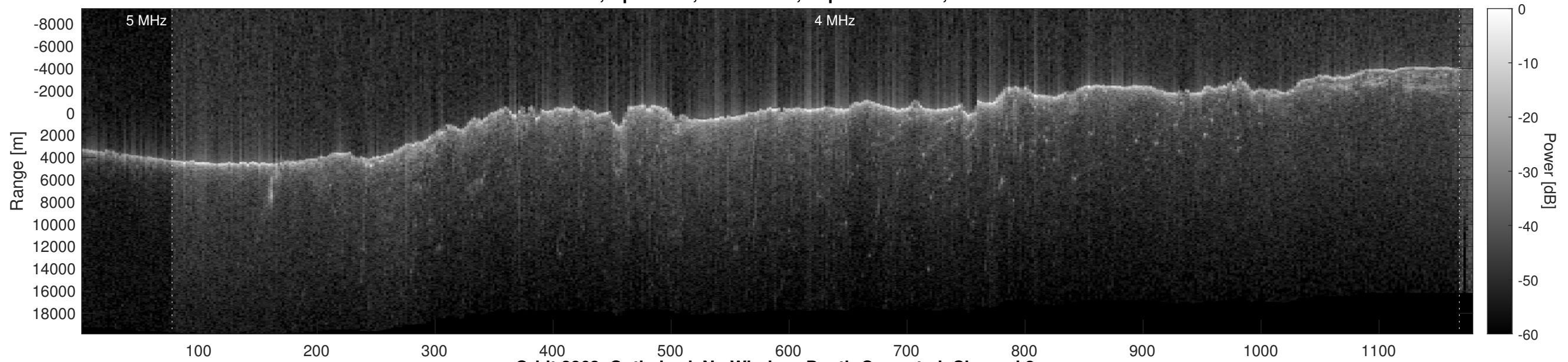
Orbit 2863, Optimized, No Window, Depth-Corrected, Channel 2
