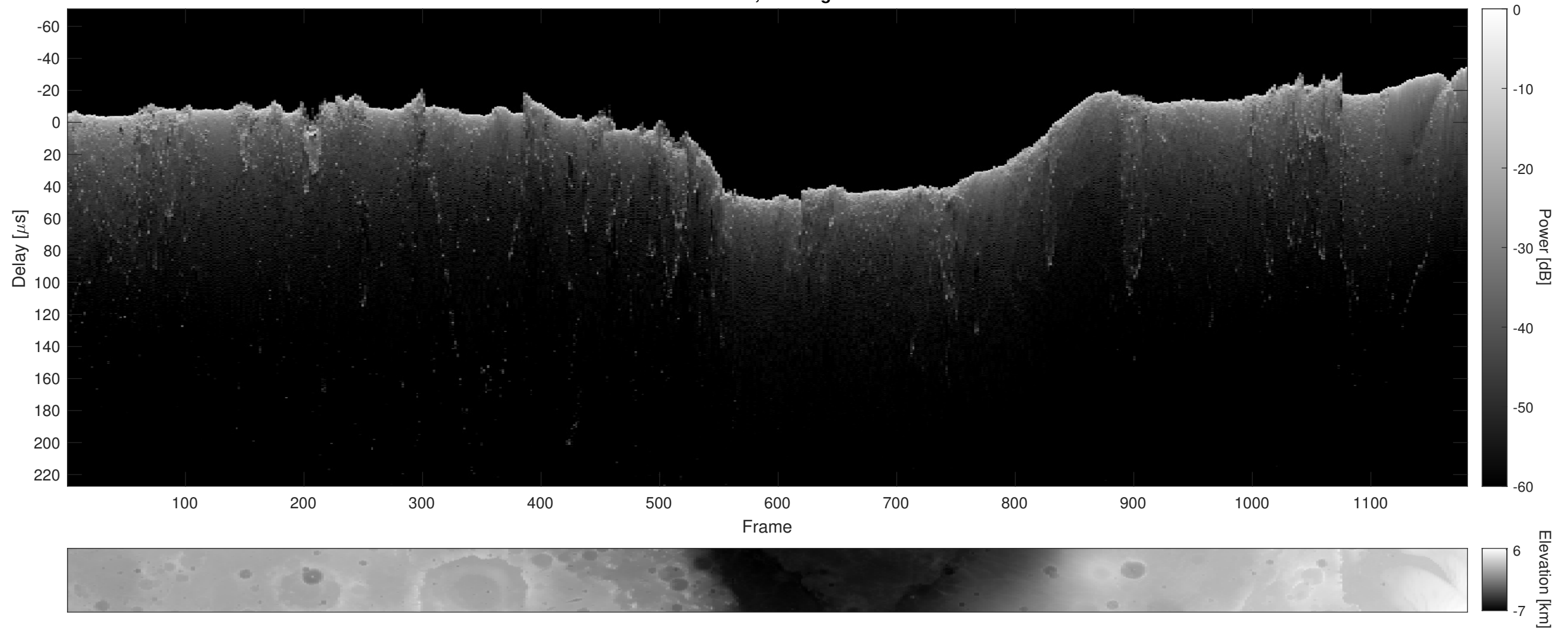
Orbit 2864, Cluttergram
