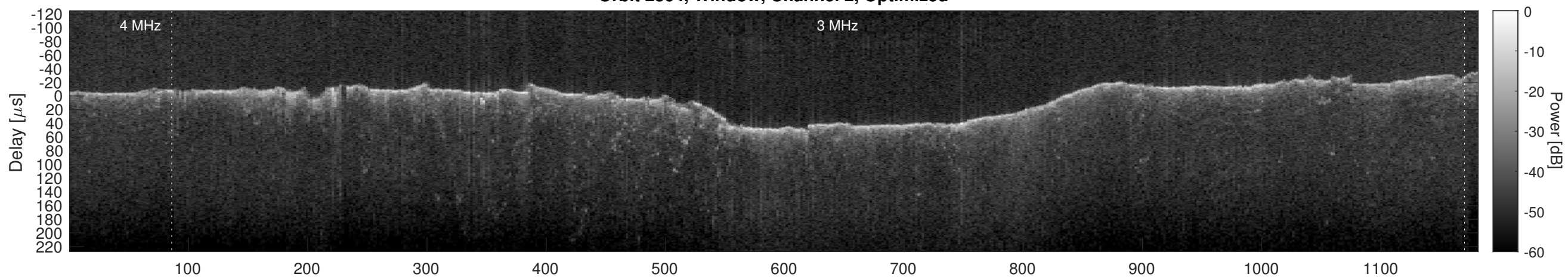
Orbit 2864, Cluttergram
