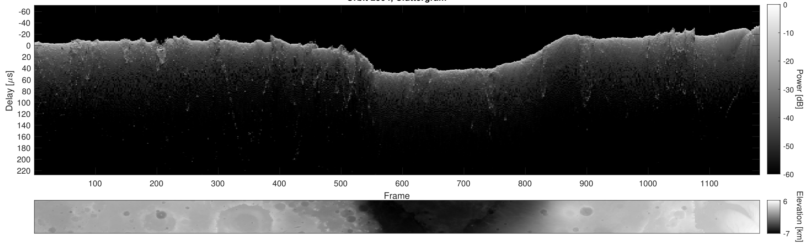
Orbit 2864, Cluttergram
