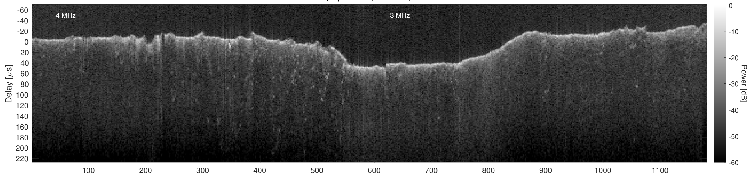
Orbit 2864, Cluttergram
