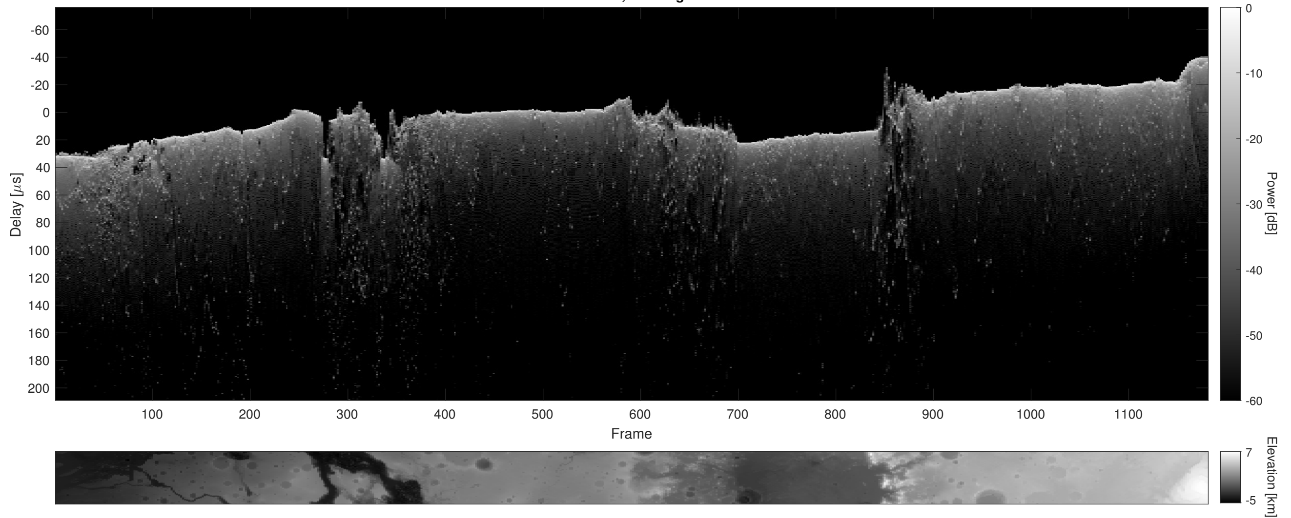
Orbit 2865, Cluttergram
