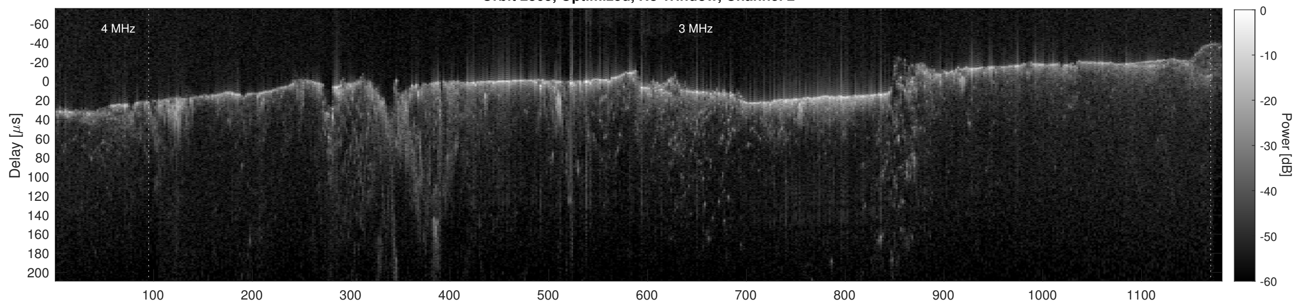
Orbit 2865, Cluttergram
