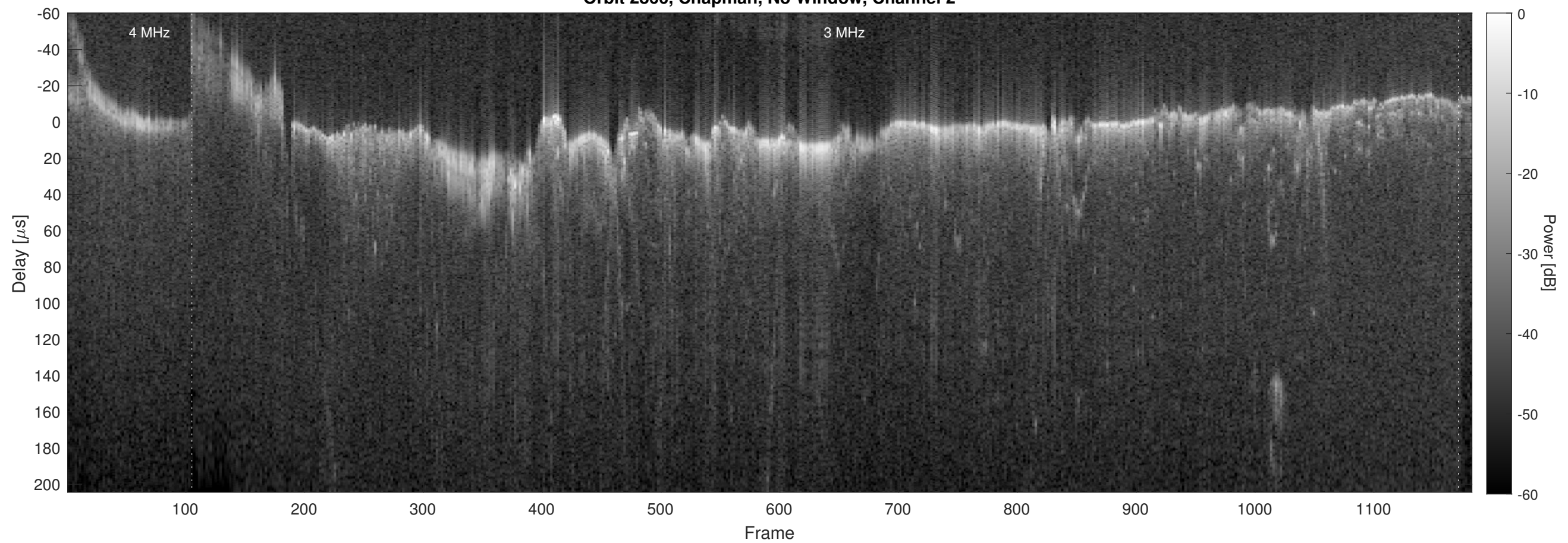
Orbit 2866, Chapman, No Window, Channel 2
