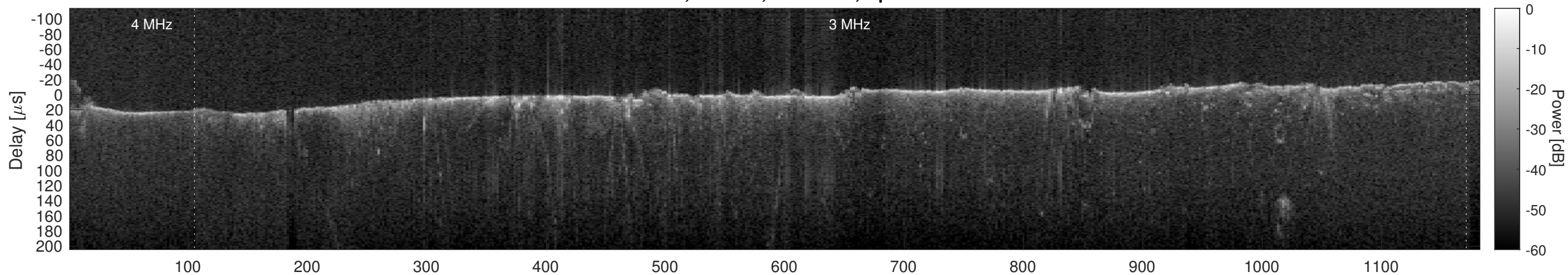
Orbit 2866, Cluttergram
