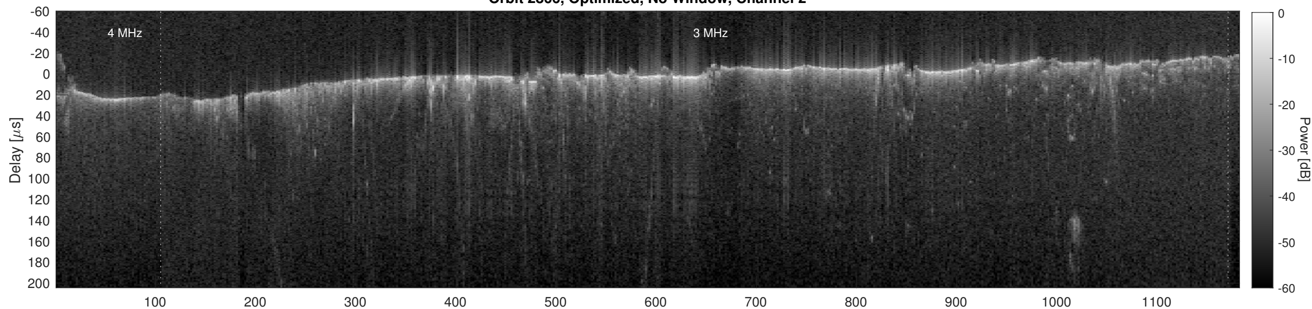
Orbit 2866, Cluttergram
