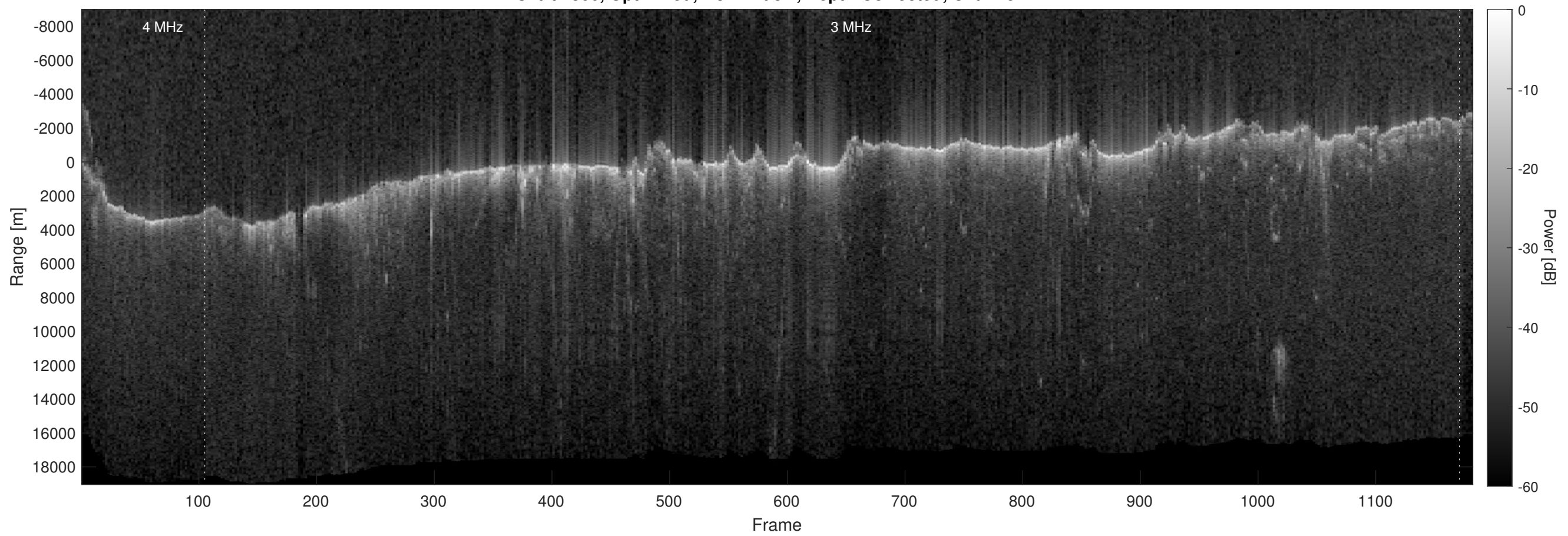
Orbit 2866, Optimized, No Window, Depth-Corrected, Channel 2
