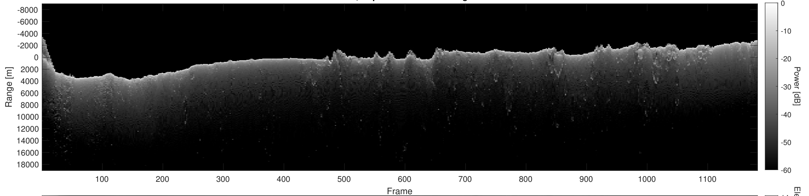
Orbit 2866, Depth-Corrected Cluttergram
