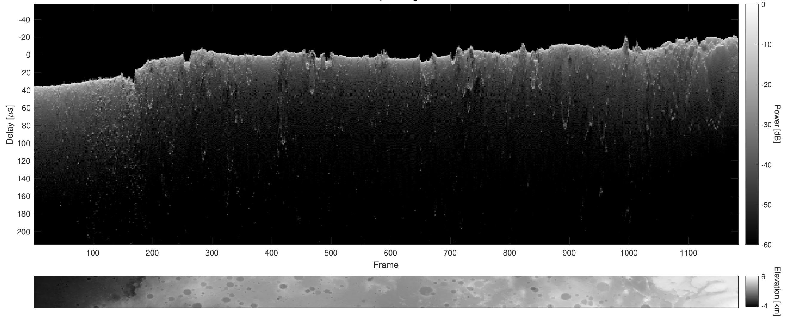
Orbit 2867, Cluttergram
