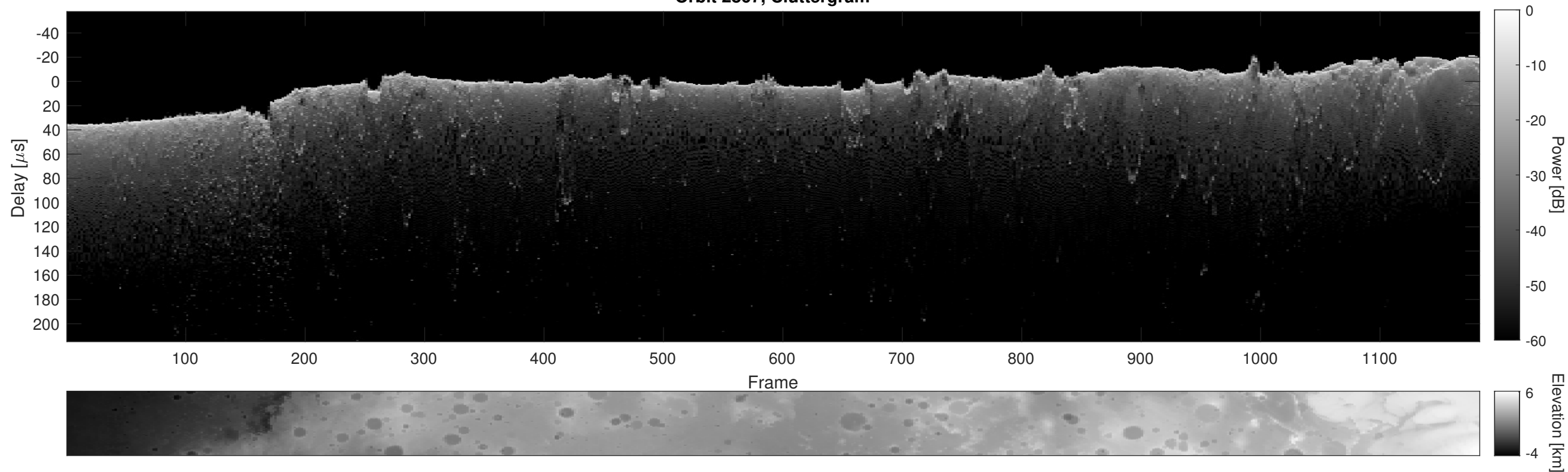
Orbit 2867, Cluttergram
