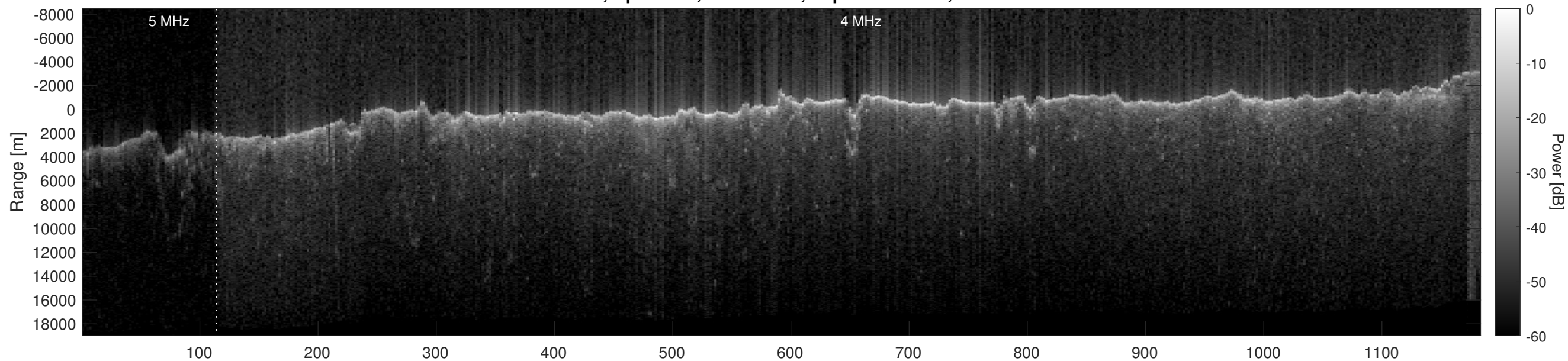
Orbit 2868, Optimized, No Window, Depth-Corrected, Channel 2
