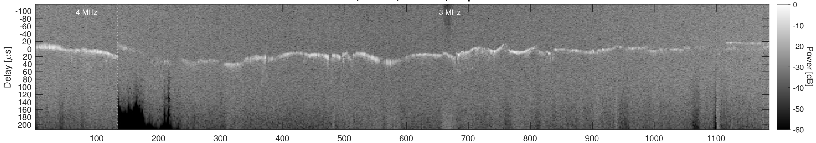
Orbit 2870, Window, Channel 2, Optimized
