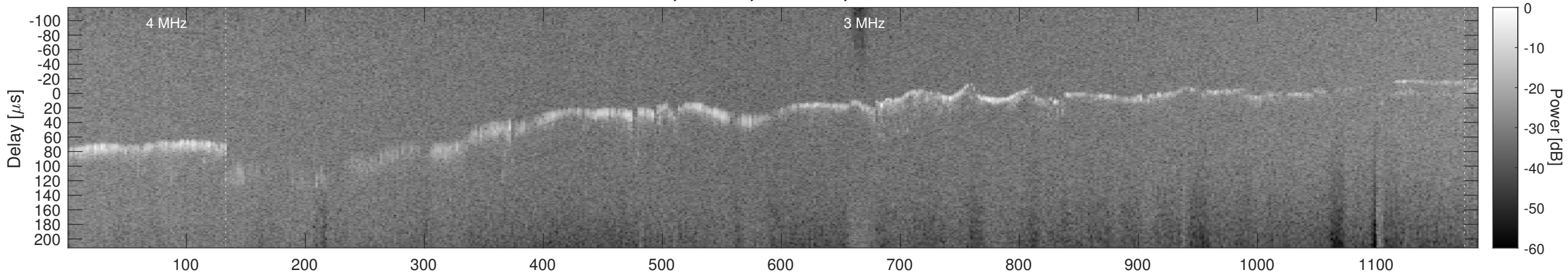
Orbit 2870, Window, Channel 2, Chapman
