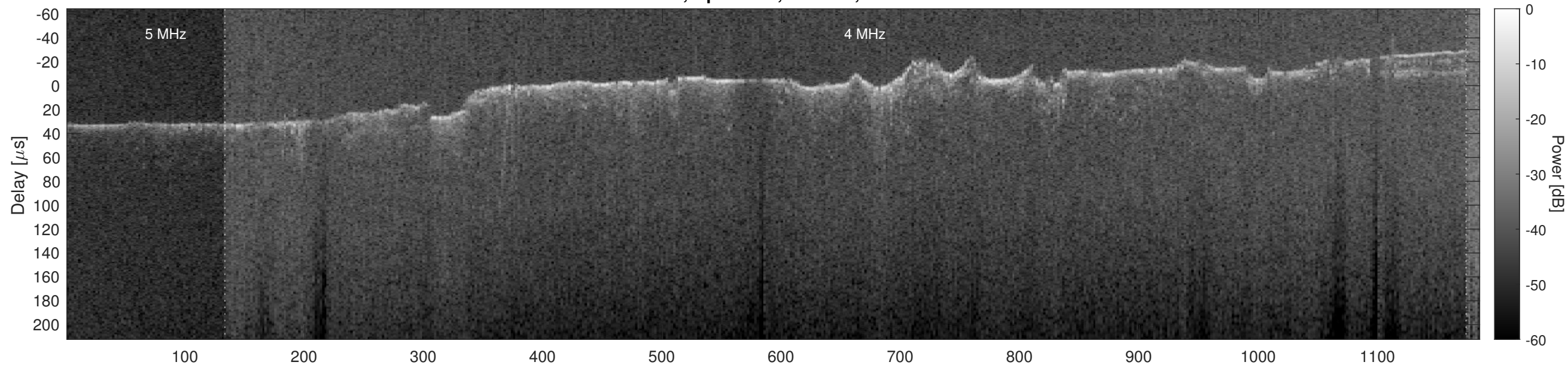
Orbit 2870, Optimized, Window, Channel 2
