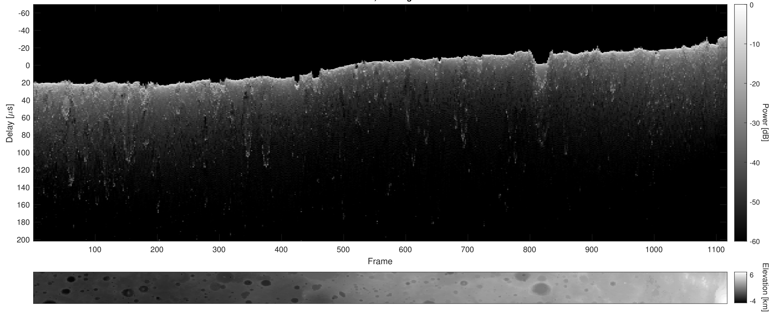
Orbit 2872, Cluttergram
