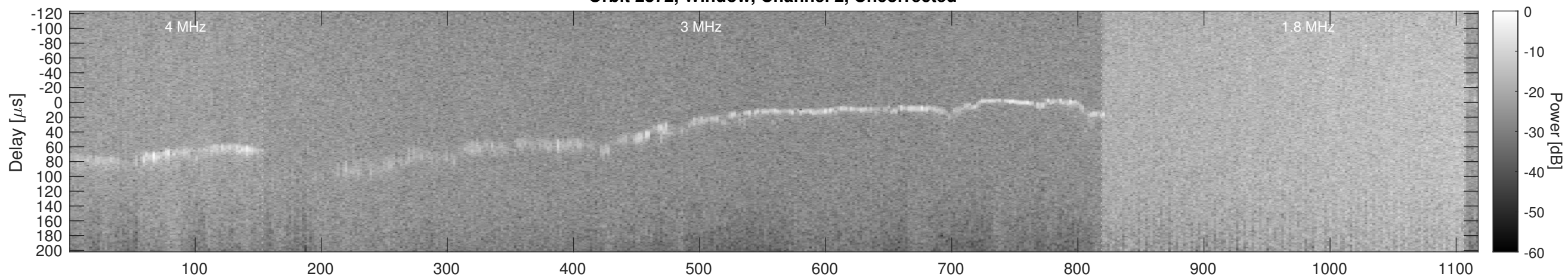
Orbit 2872, Window, Channel 2, Chapman
