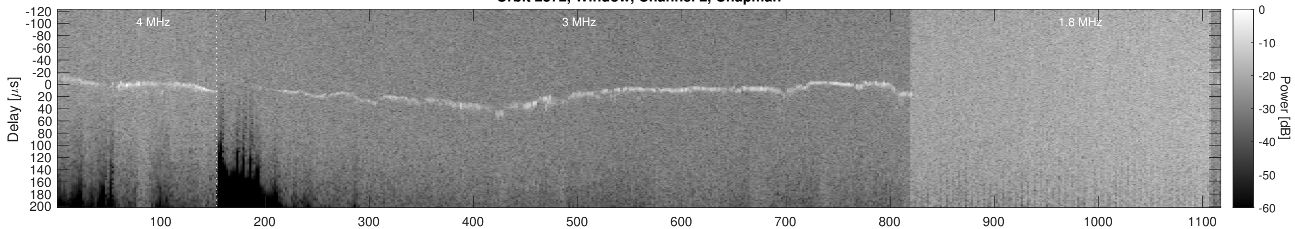
Orbit 2872, Window, Channel 2, Optimized
