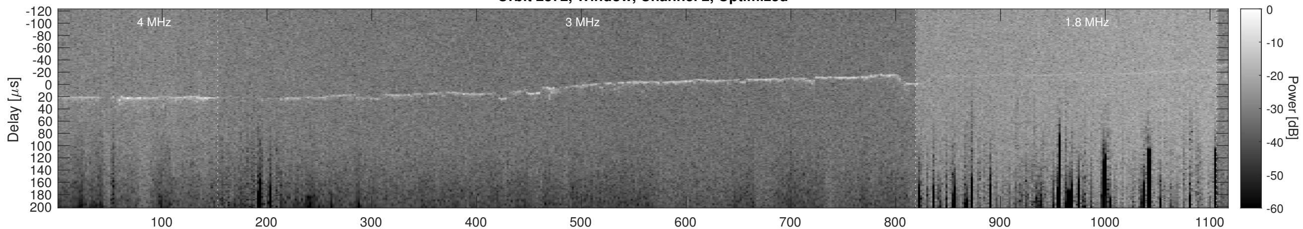
Orbit 2872, Cluttergram
