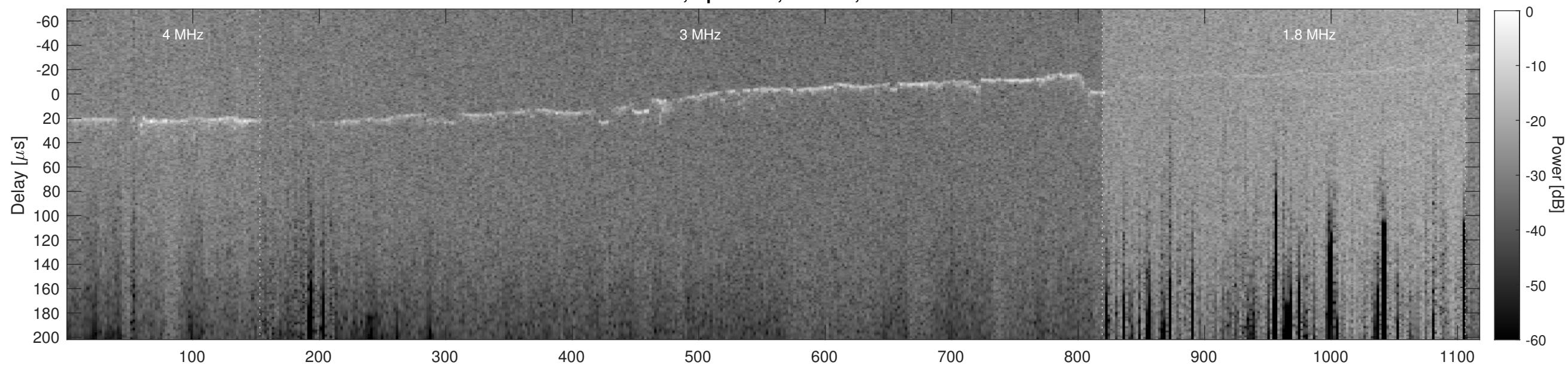
Orbit 2872, Cluttergram
