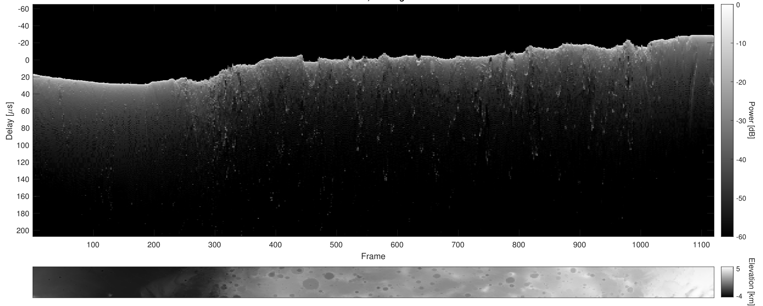
Orbit 2874, Cluttergram
