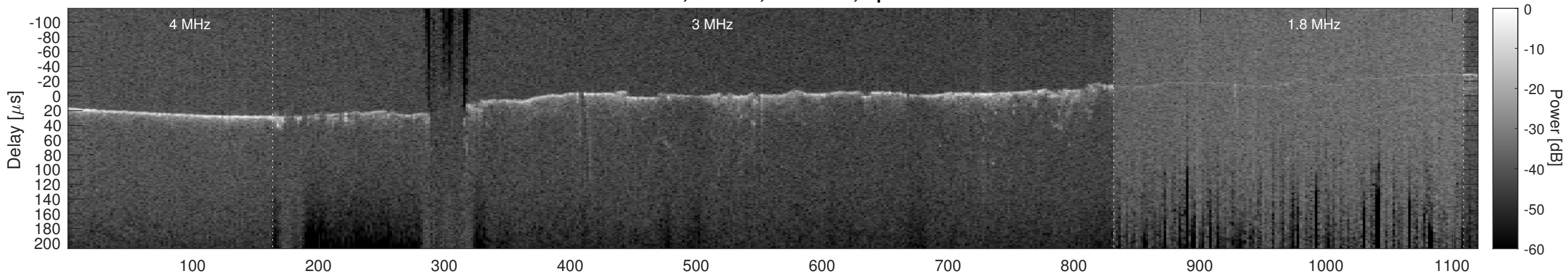
Orbit 2874, Cluttergram
