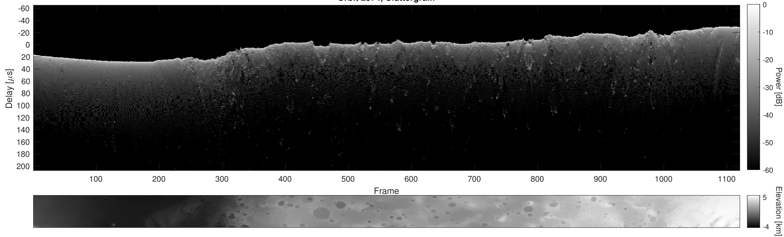
Orbit 2874, Cluttergram
