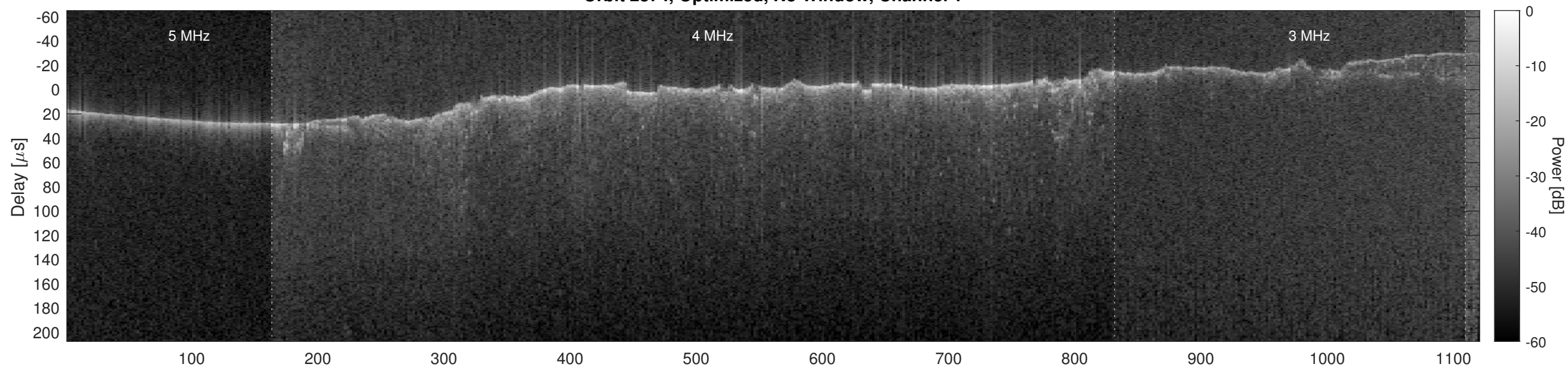
Orbit 2874, Optimized, No Window, Channel 2
