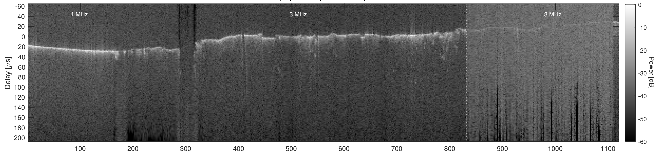
Orbit 2874, Cluttergram
