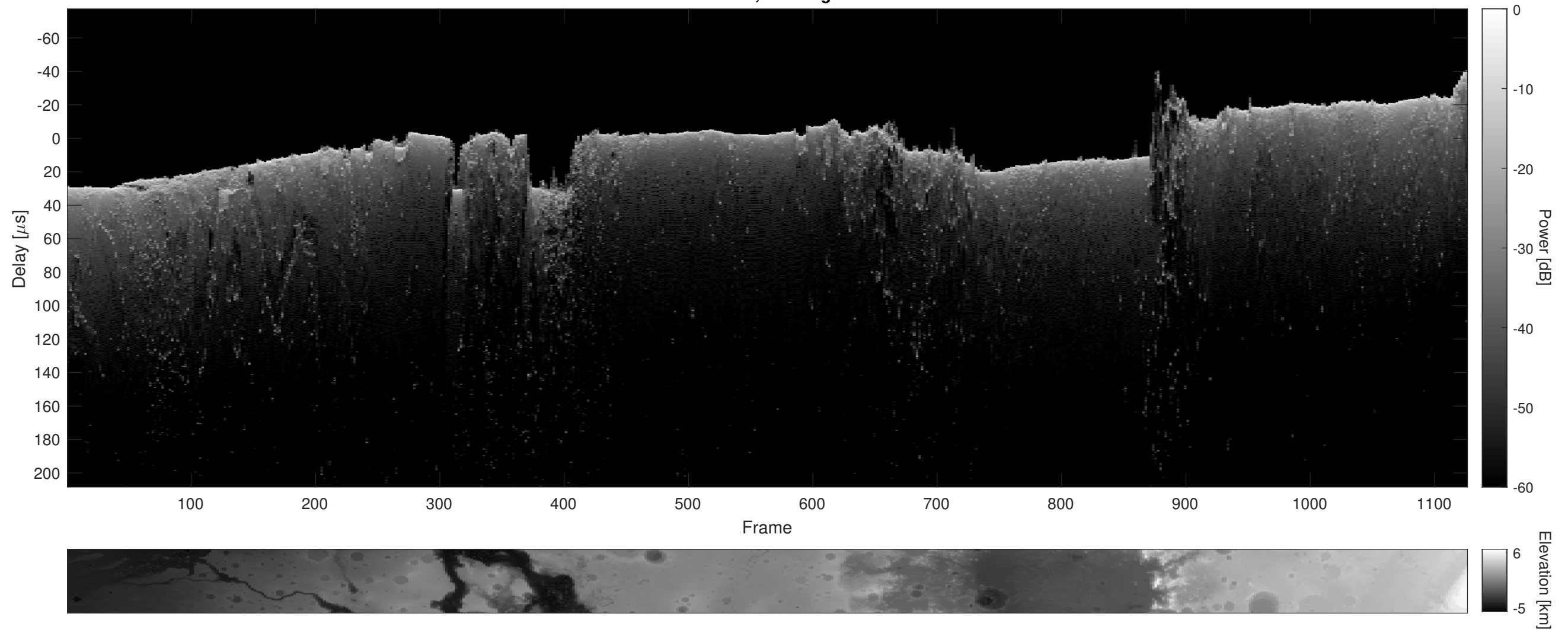
Orbit 2876, Cluttergram
