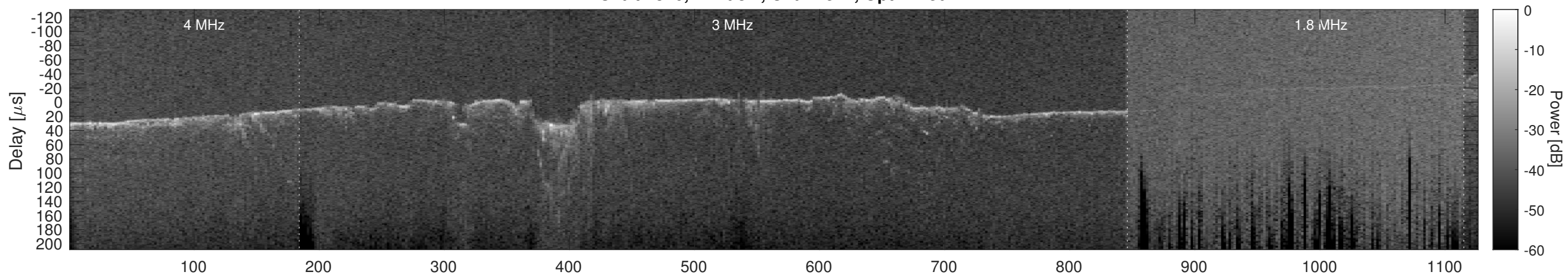
Orbit 2876, Cluttergram
