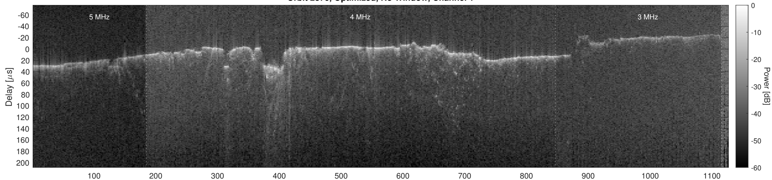
Orbit 2876, Optimized, No Window, Channel 2
