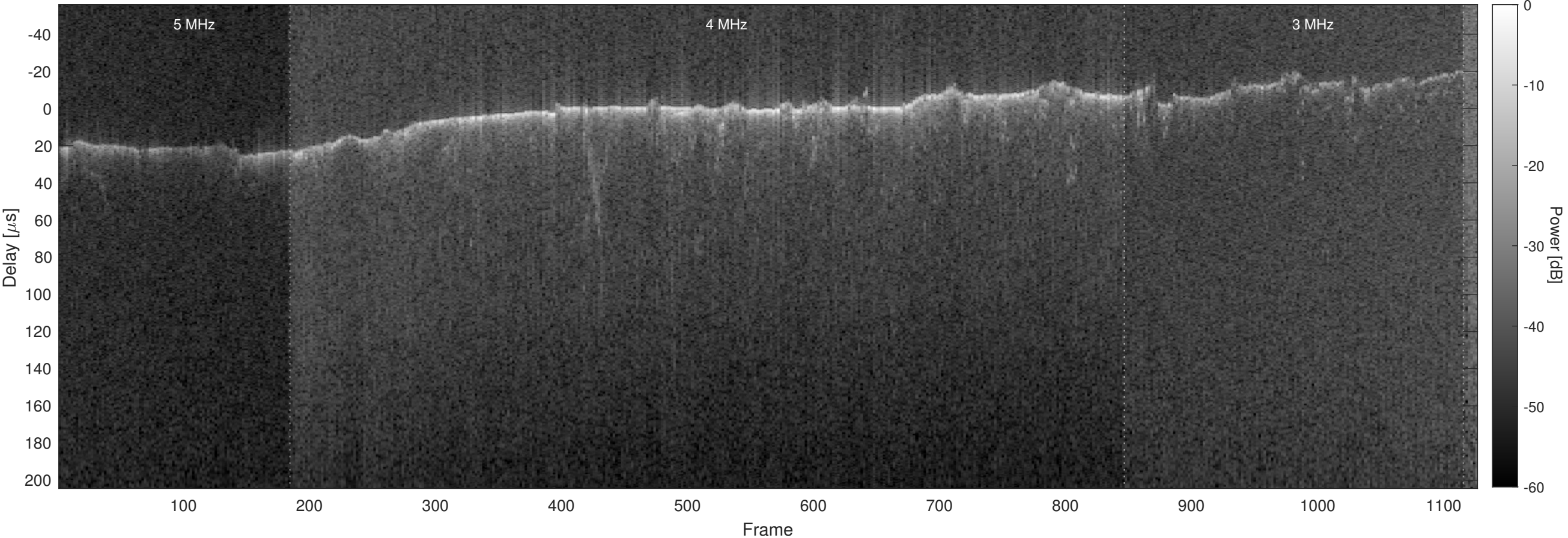
Orbit 2877, Optimized, No Window, Channel 2
