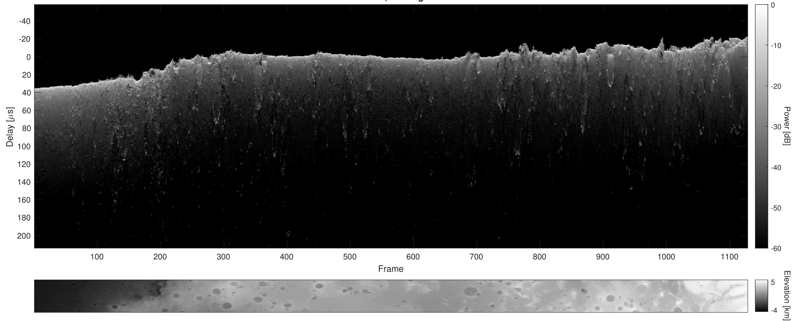
Orbit 2878, Cluttergram
