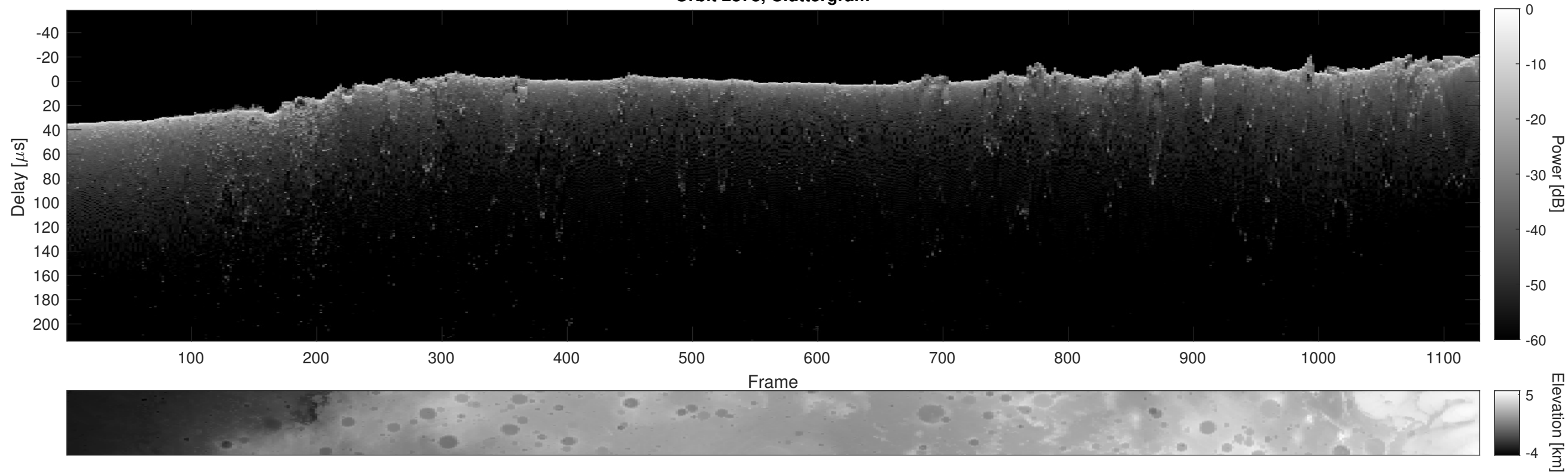
Orbit 2878, Cluttergram
