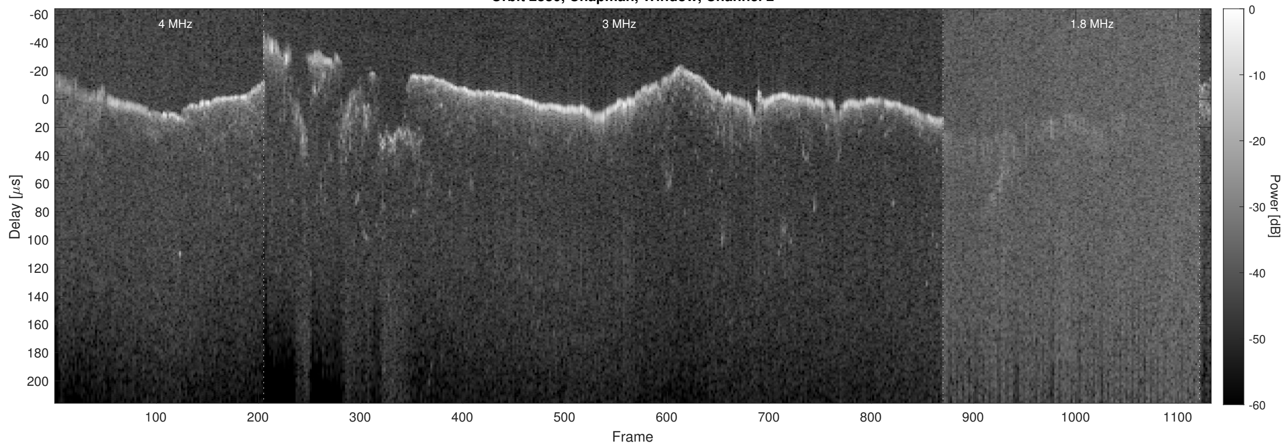
Orbit 2880, Chapman, Window, Channel 2
