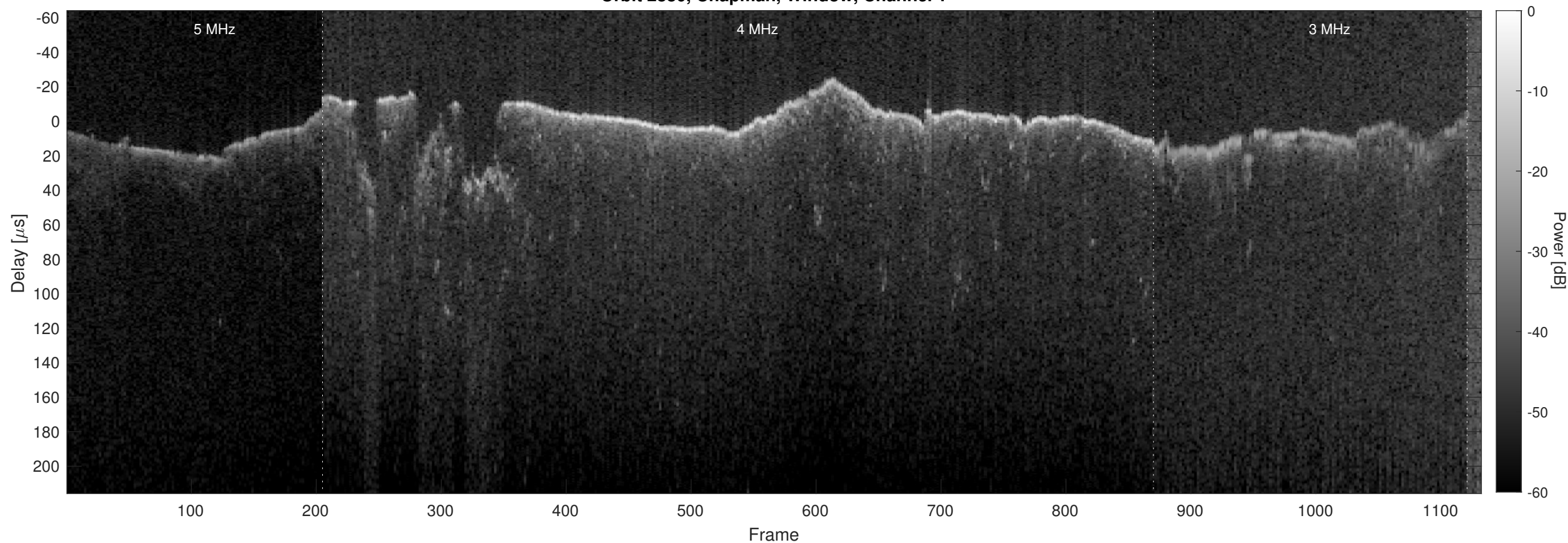
Orbit 2880, Chapman, Window, Channel 2
