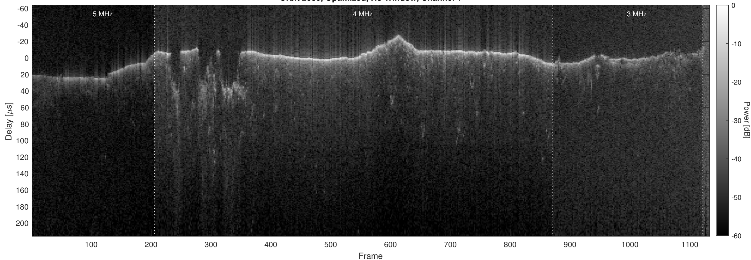
Orbit 2880, Optimized, No Window, Channel 2
