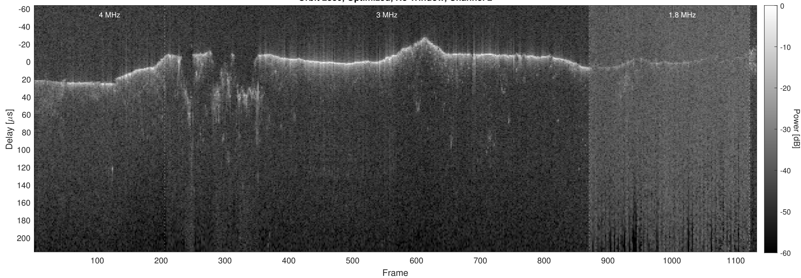
Orbit 2880, Optimized, No Window, Channel 2
