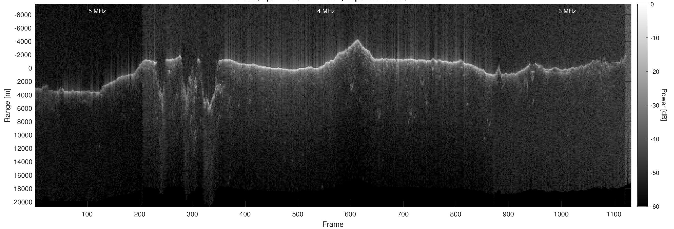
Orbit 2880, Optimized, No Window, Depth-Corrected, Channel 2
