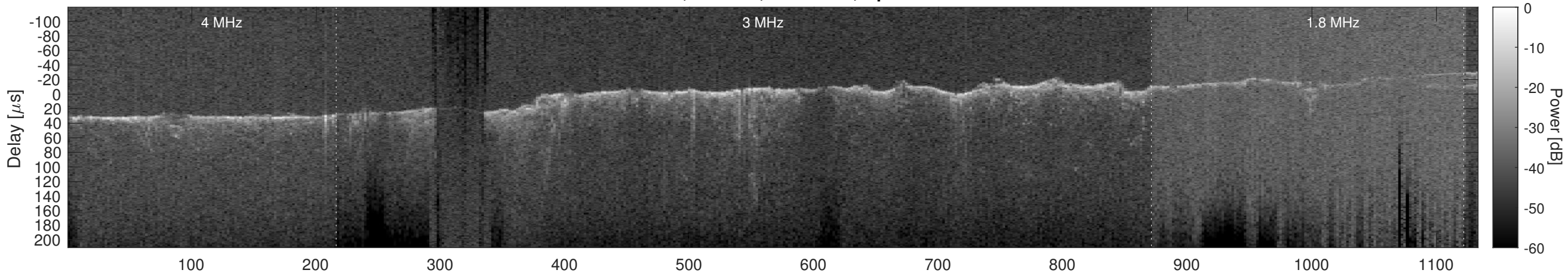
Orbit 2881, Cluttergram
