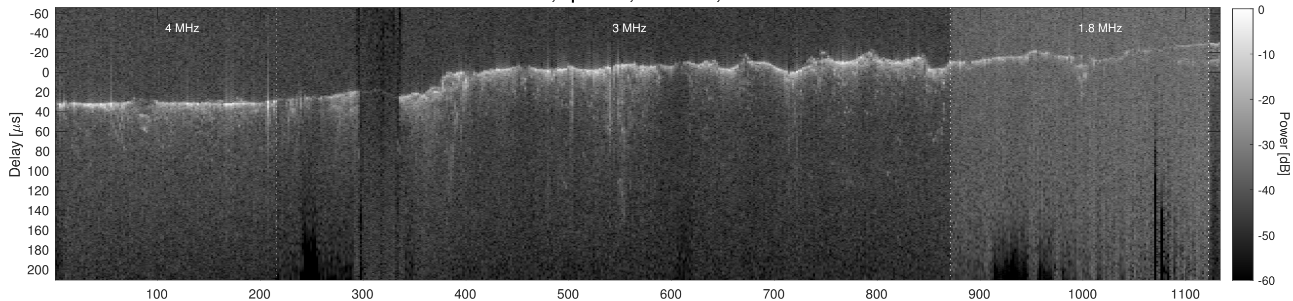
Orbit 2881, Cluttergram
