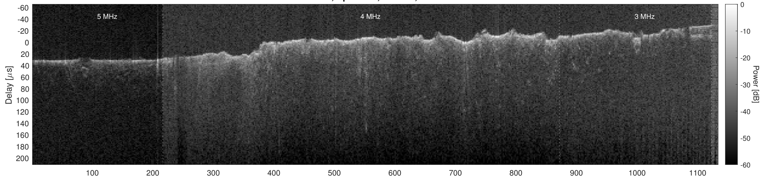
Orbit 2881, Optimized, Window, Channel 2
