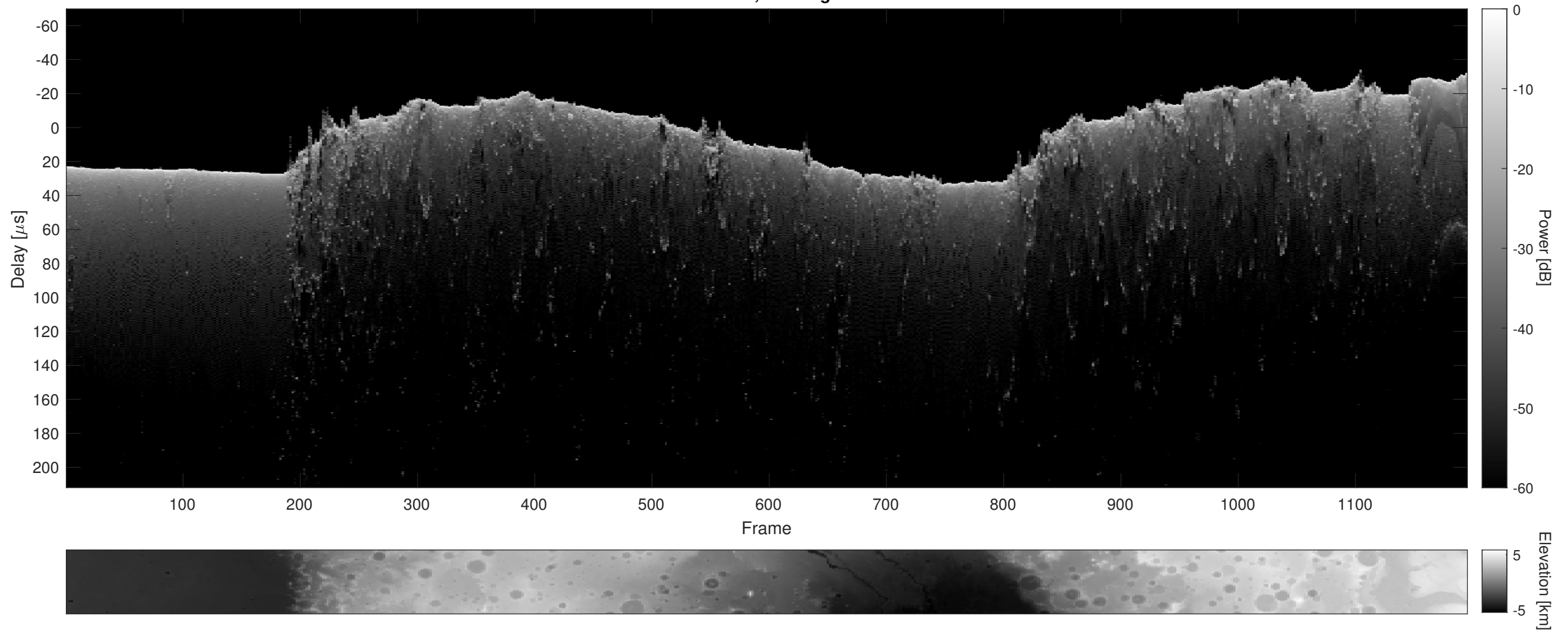
Orbit 2882, Cluttergram
